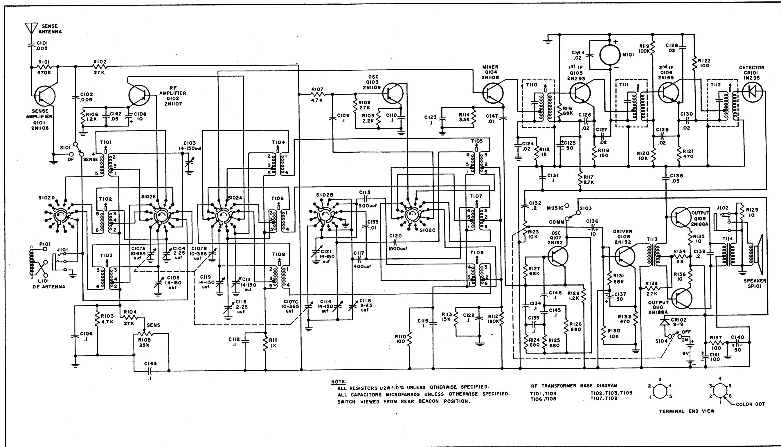
Figure 11. Schematic Diagram
